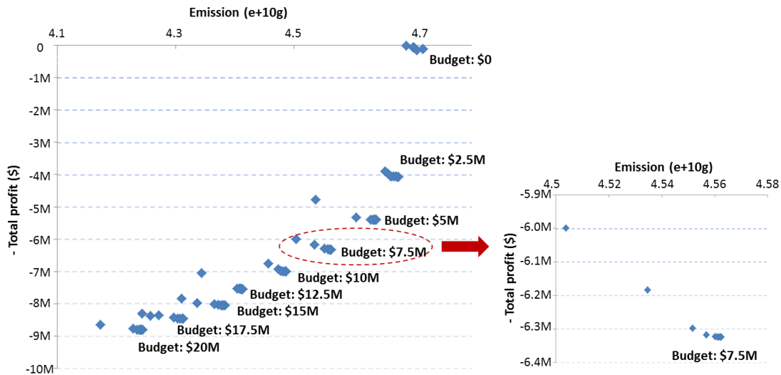
Figure 6. Pareto curves for the all-in-one scenario
