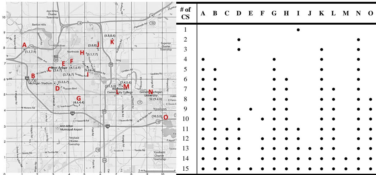
Figure 3. Optimal charging station locations using candidates (A to O)
